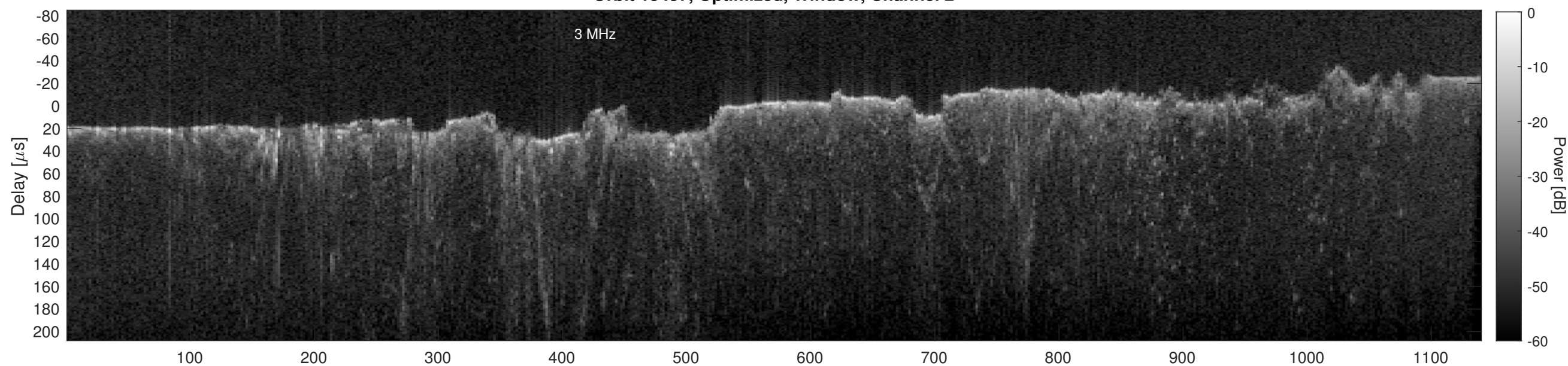
Orbit 15457, Cluttergram
