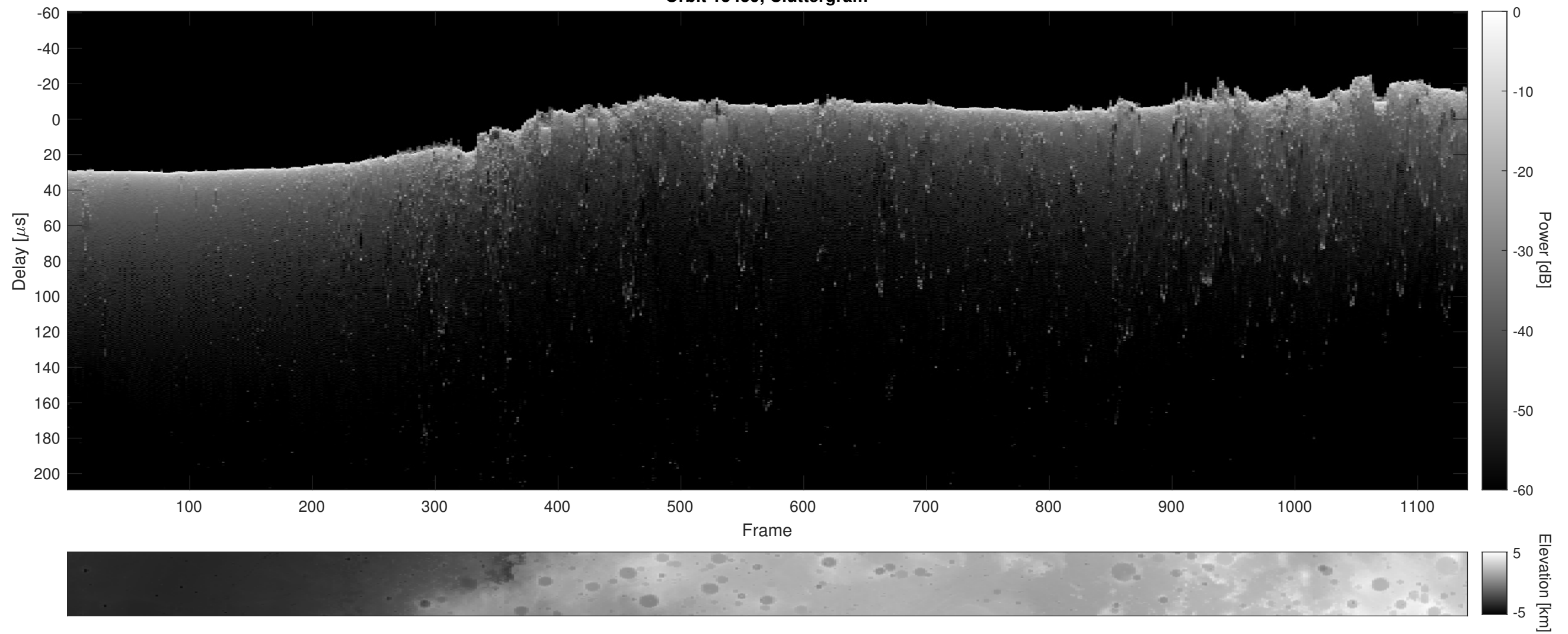
Orbit 15459, Cluttergram
