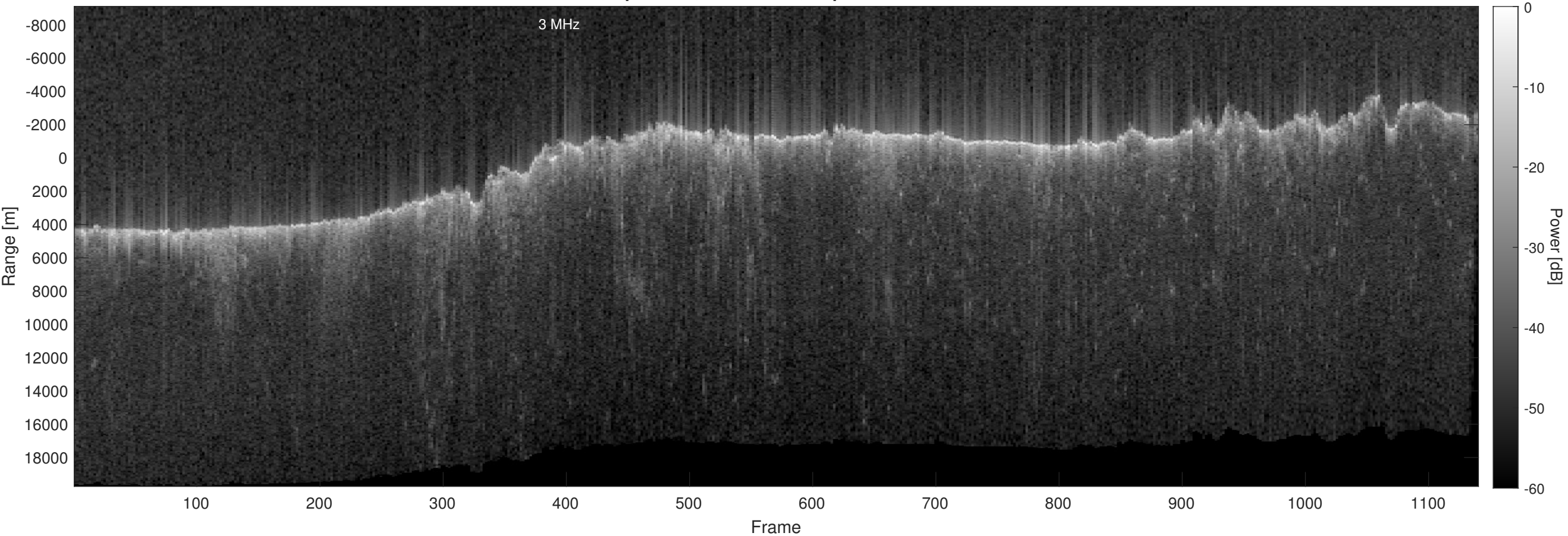
Orbit 15459, Optimized, No Window, Depth-Corrected, Channel 2
