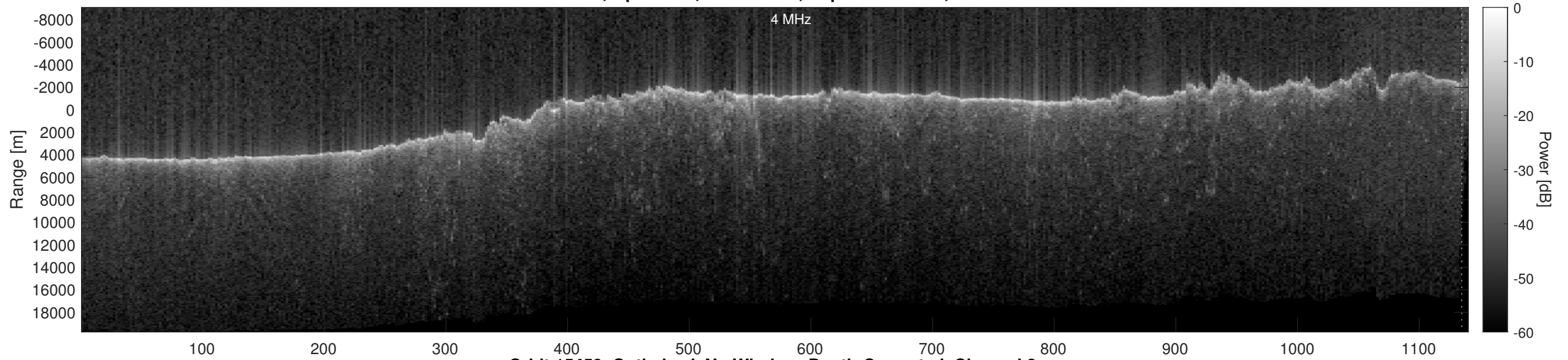
Orbit 15459, Optimized, No Window, Depth-Corrected, Channel 2
