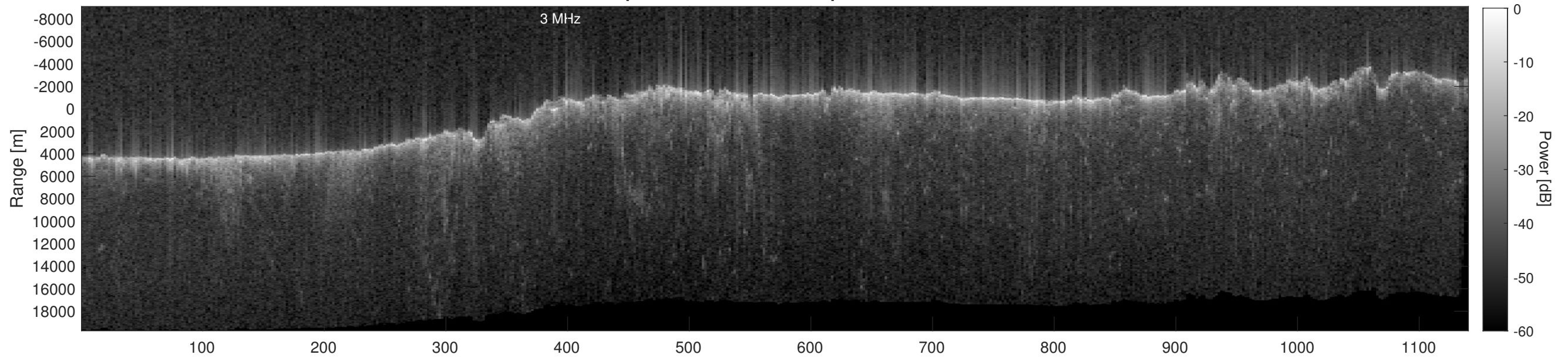
Orbit 15459, Depth-Corrected Cluttergram
