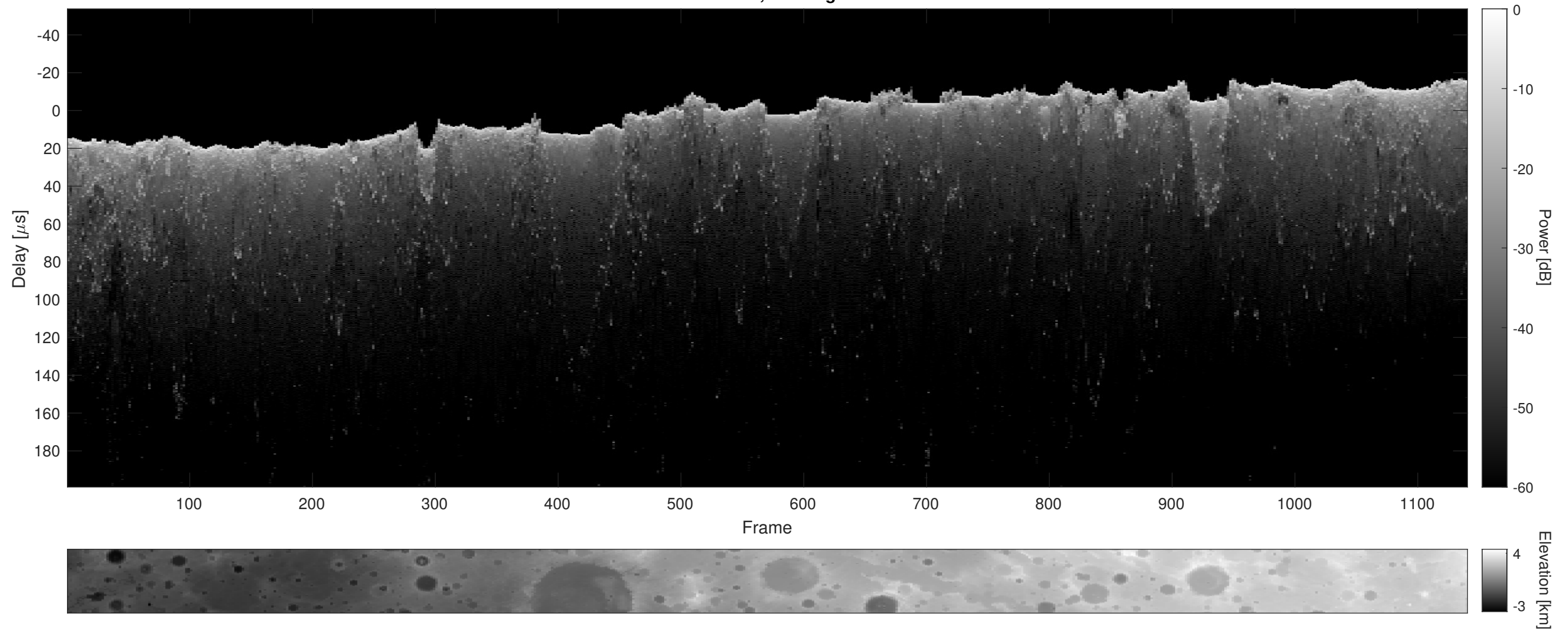
Orbit 15460, Cluttergram
