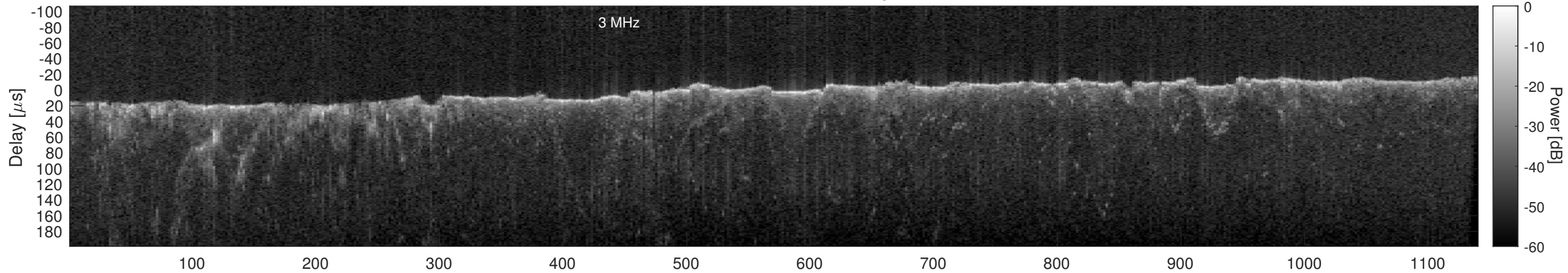
Orbit 15460, Cluttergram
