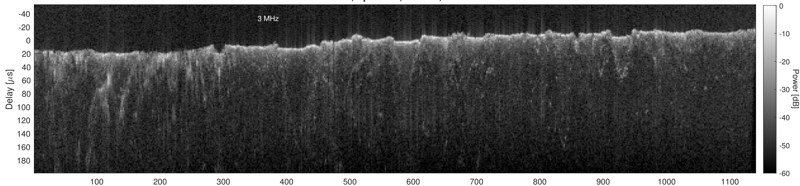
Orbit 15460, Cluttergram
