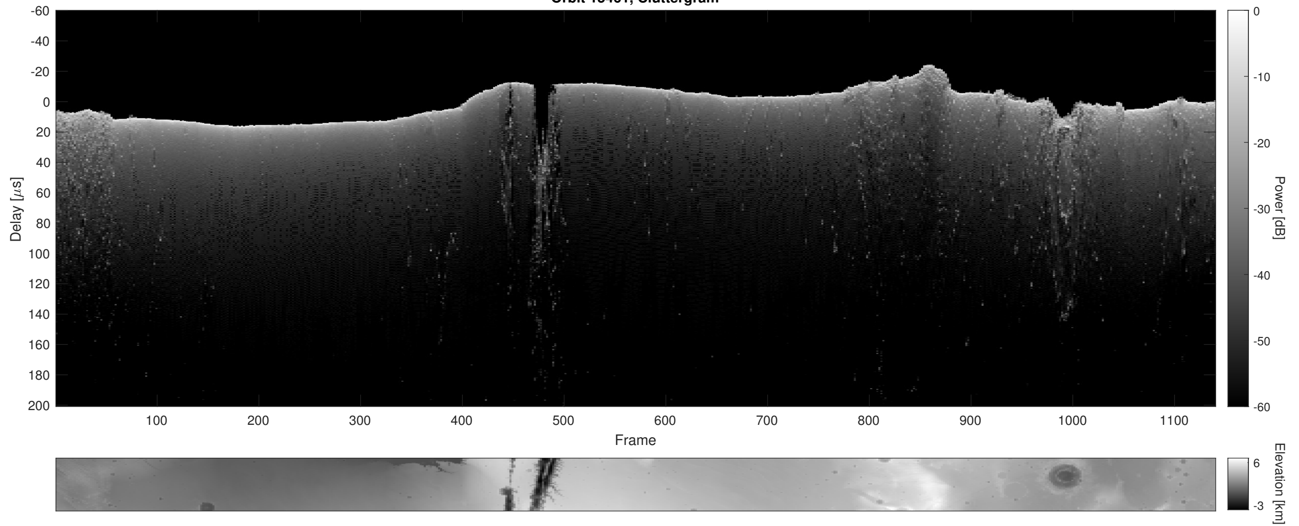
Orbit 15461, Cluttergram
