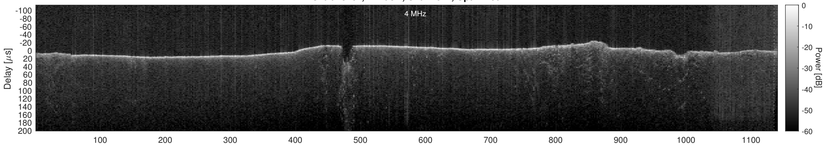
Orbit 15461, Cluttergram
