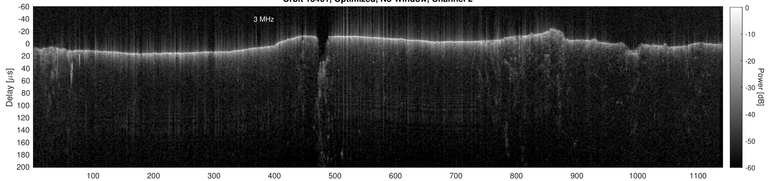
Orbit 15461, Cluttergram
