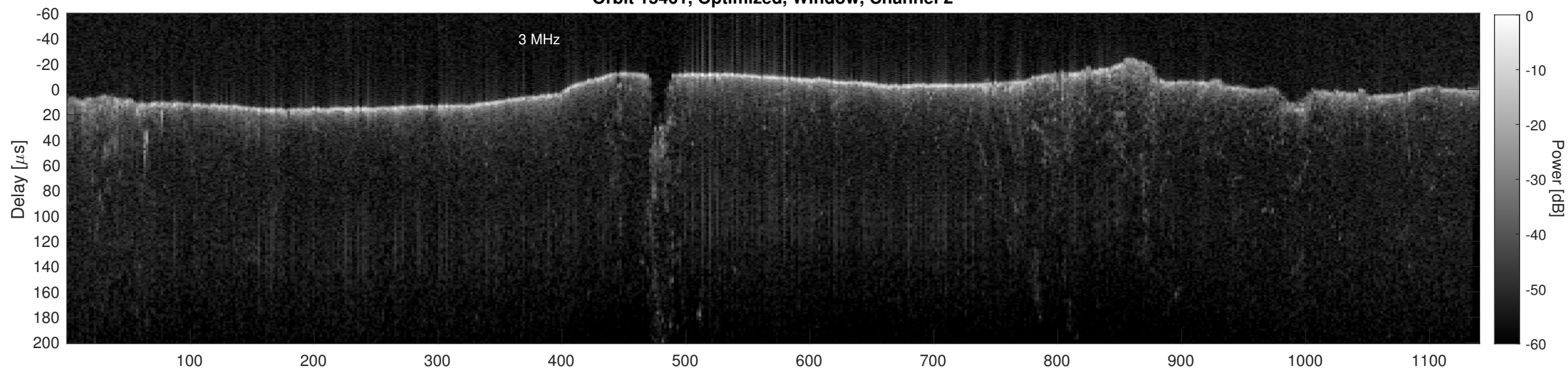
Orbit 15461, Cluttergram
