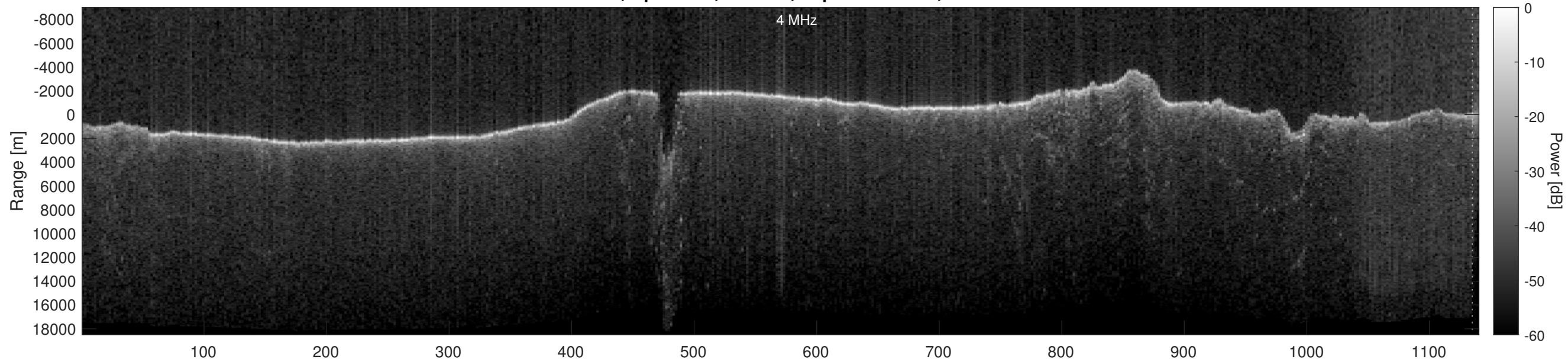
Orbit 15461, Optimized, Window, Depth-Corrected, Channel 2
