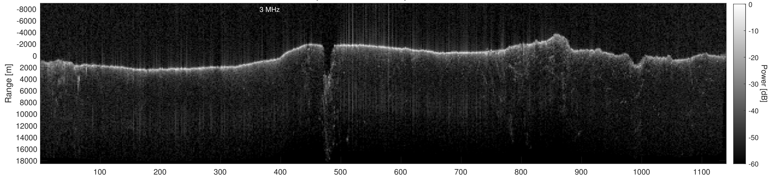
Orbit 15461, Depth-Corrected Cluttergram
