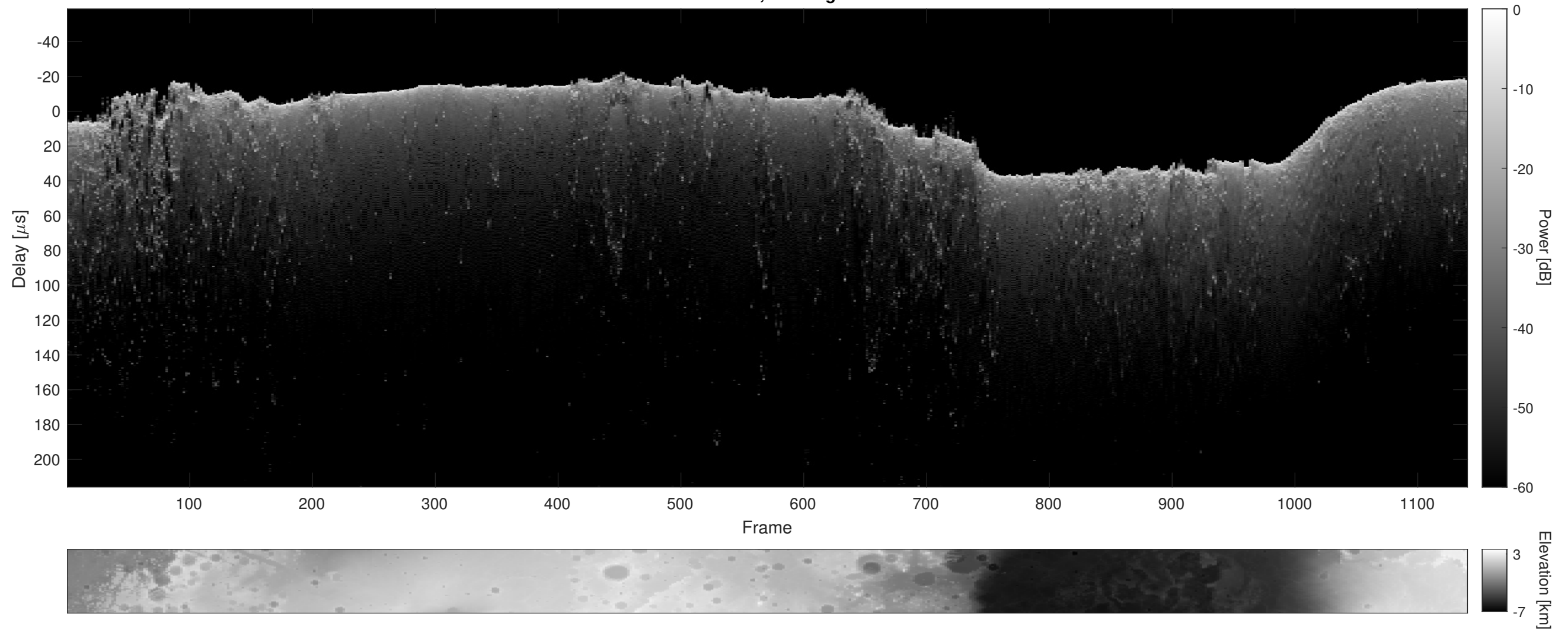
Orbit 15463, Cluttergram
