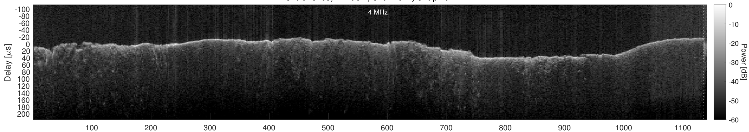
Orbit 15463, Window, Channel 1, Optimized
