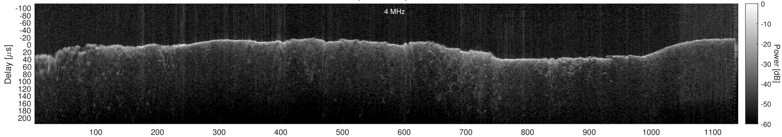
Orbit 15463, Window, Channel 1, Chapman
