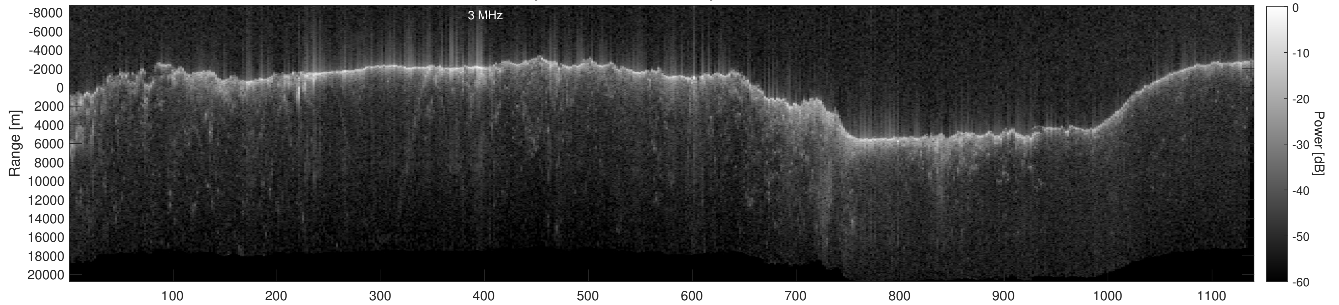
Orbit 15463, Depth-Corrected Cluttergram
