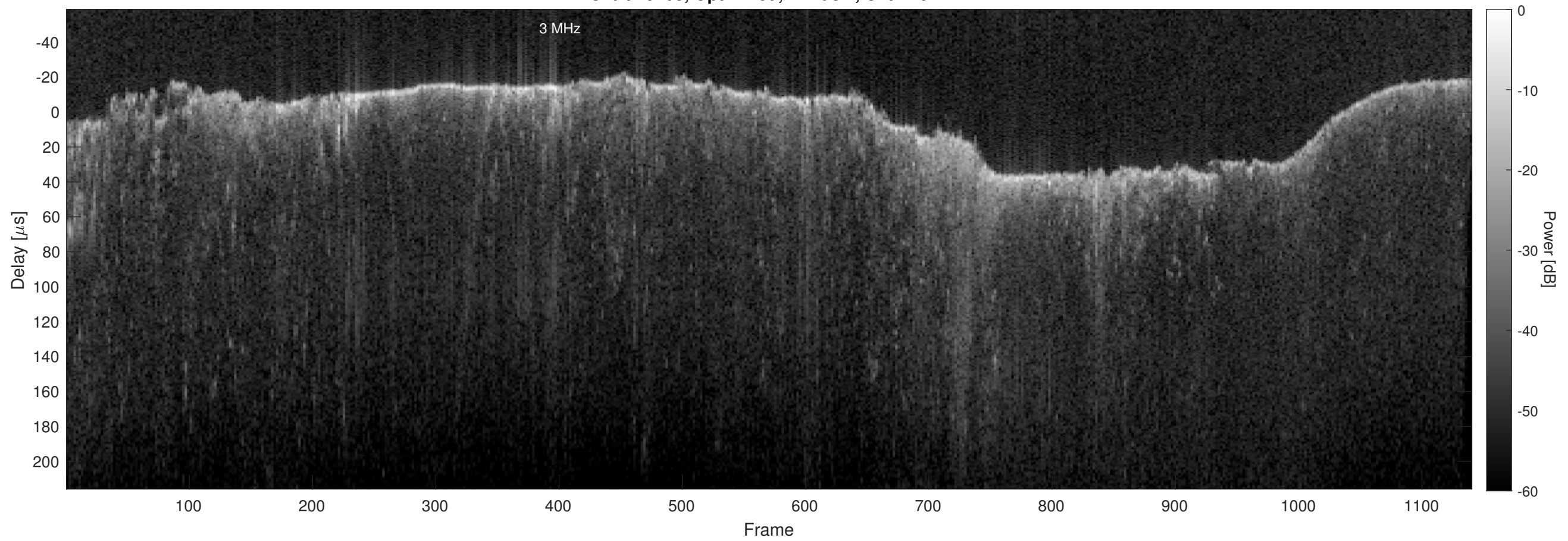
Orbit 15463, Optimized, Window, Channel 2
