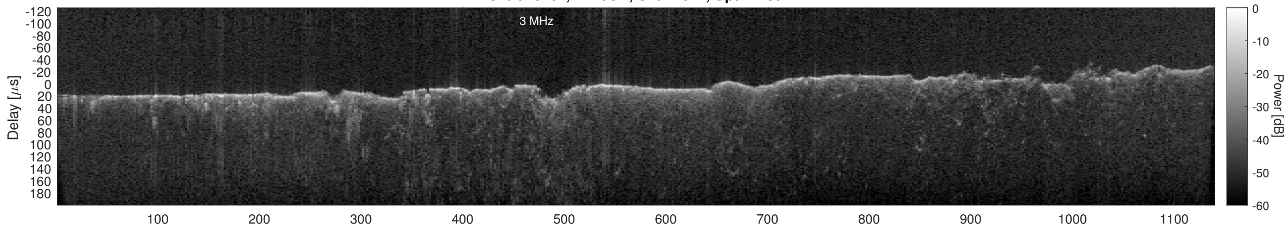
Orbit 15464, Cluttergram
