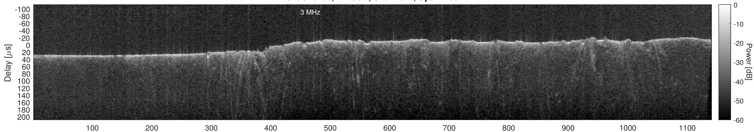
Orbit 15466, Cluttergram
