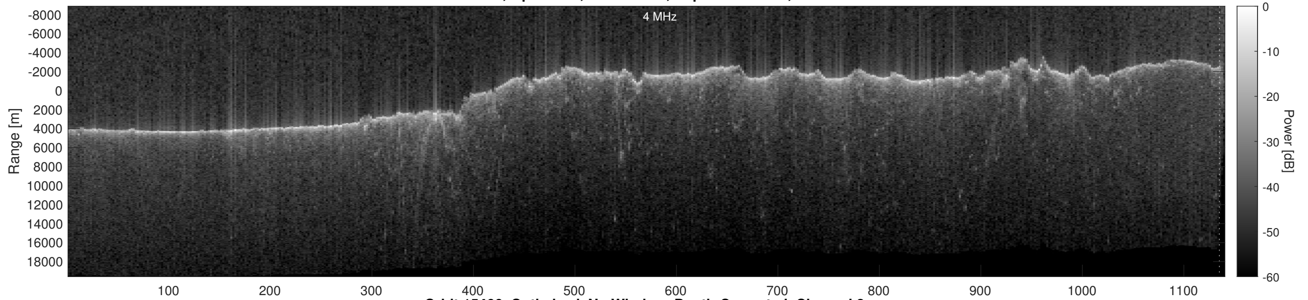
Orbit 15466, Optimized, No Window, Depth-Corrected, Channel 2
