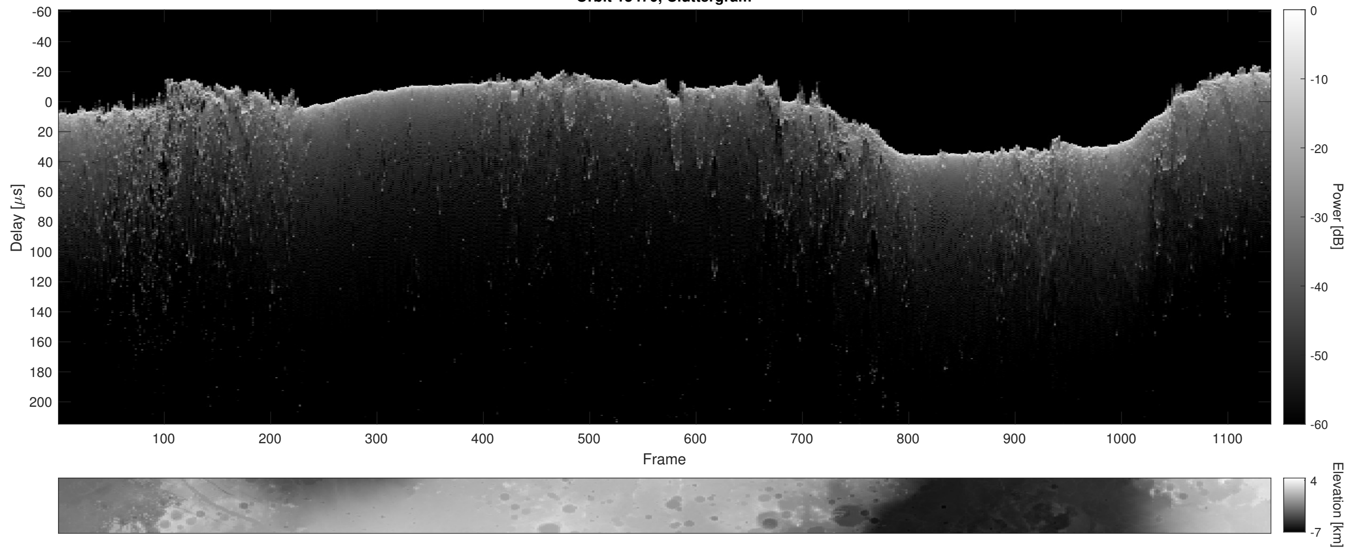
Orbit 15470, Cluttergram
