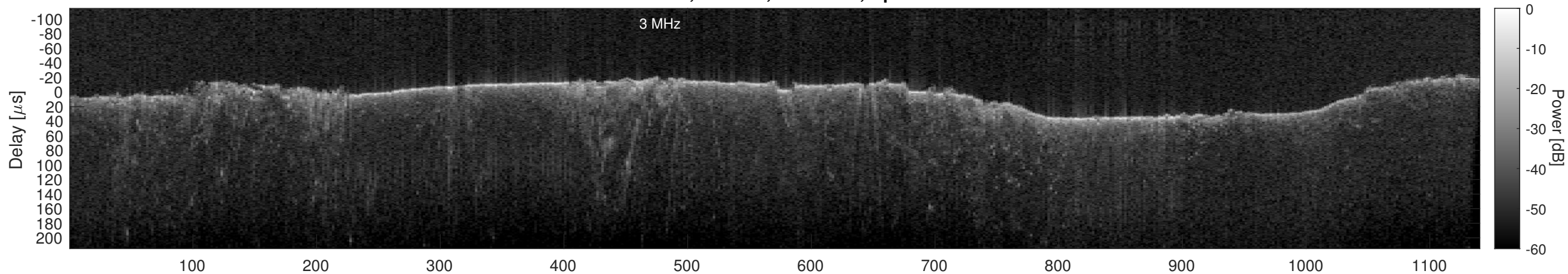
Orbit 15470, Cluttergram
