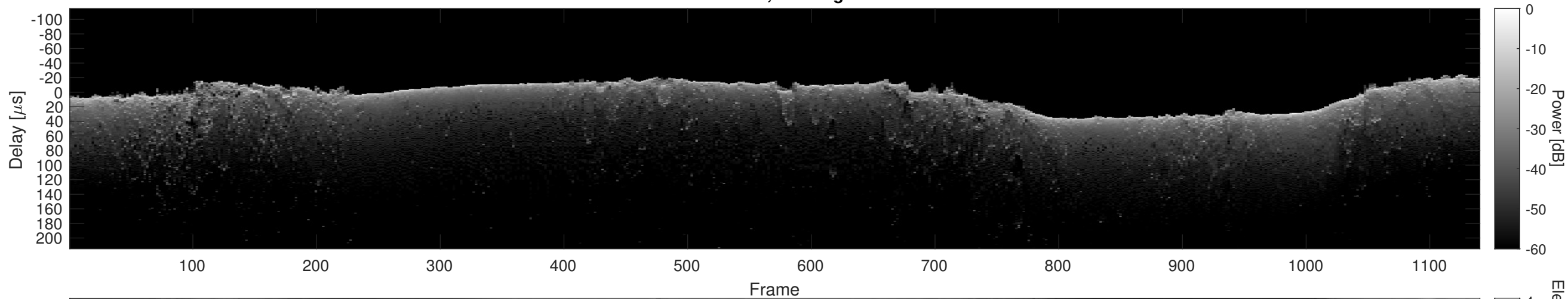
Orbit 15470, Cluttergram
