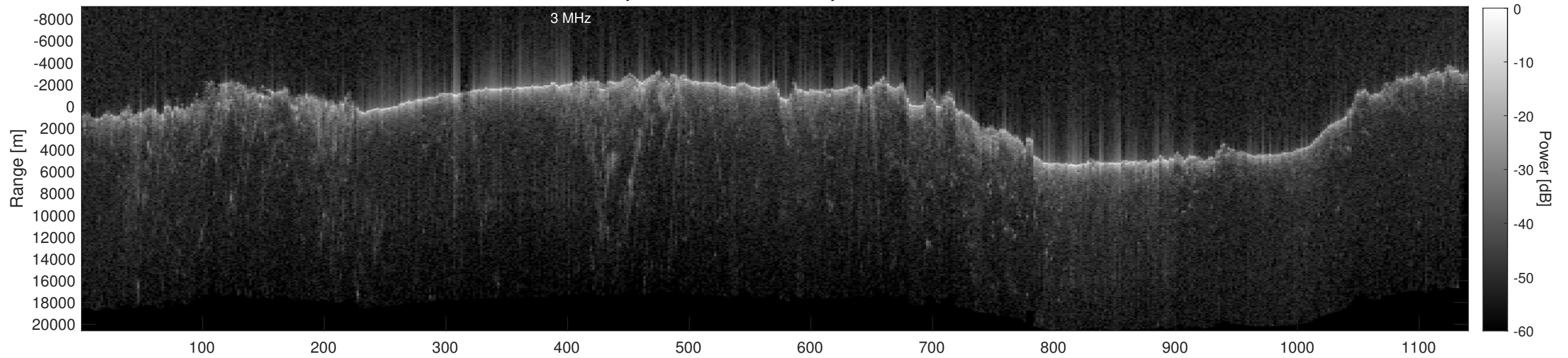
Orbit 15470, Depth-Corrected Cluttergram
