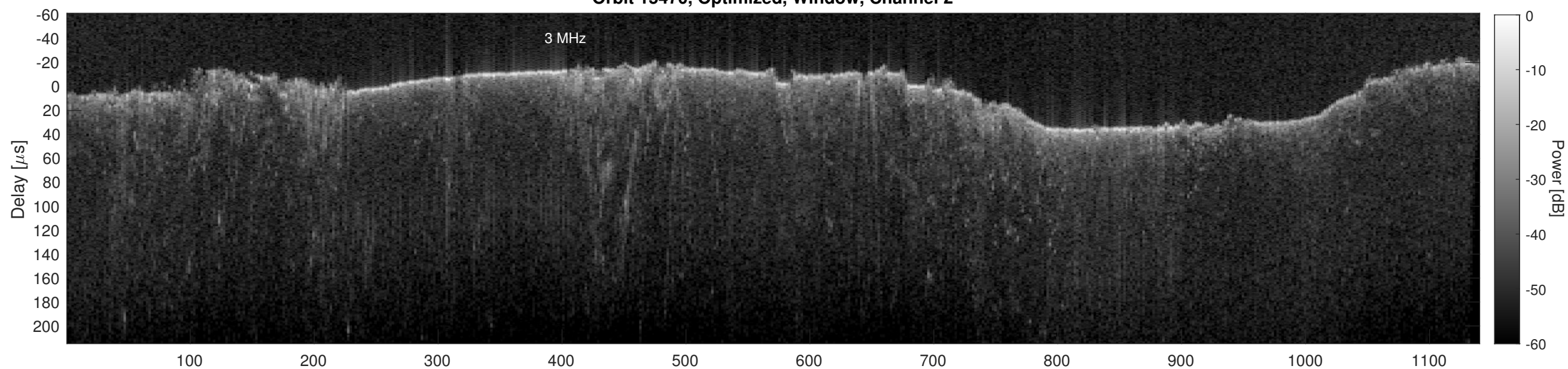
Orbit 15470, Cluttergram
