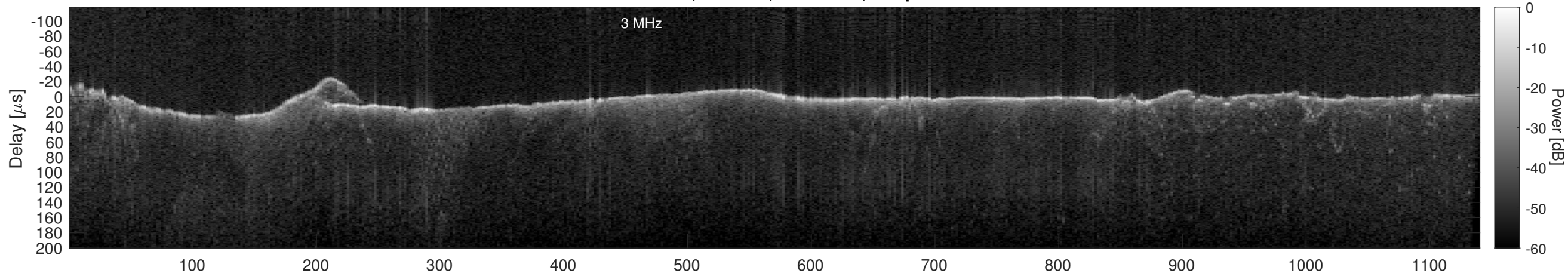
Orbit 15472, Window, Channel 2, Optimized
