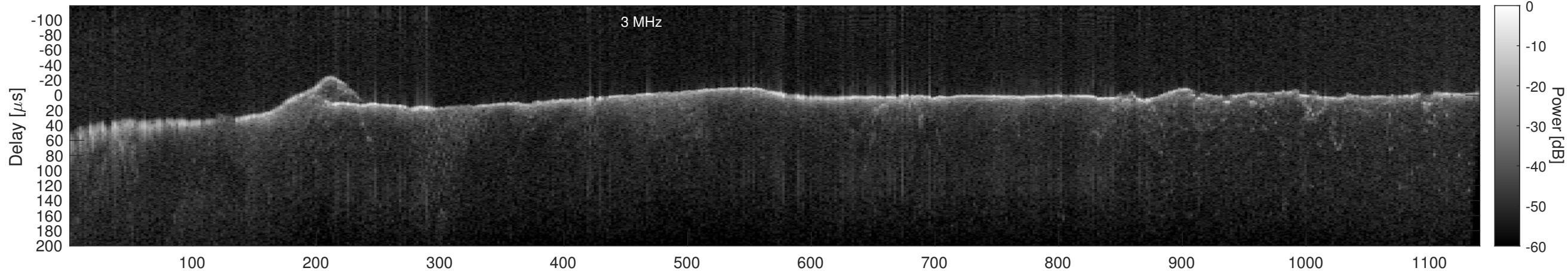
Orbit 15472, Window, Channel 2, Chapman
