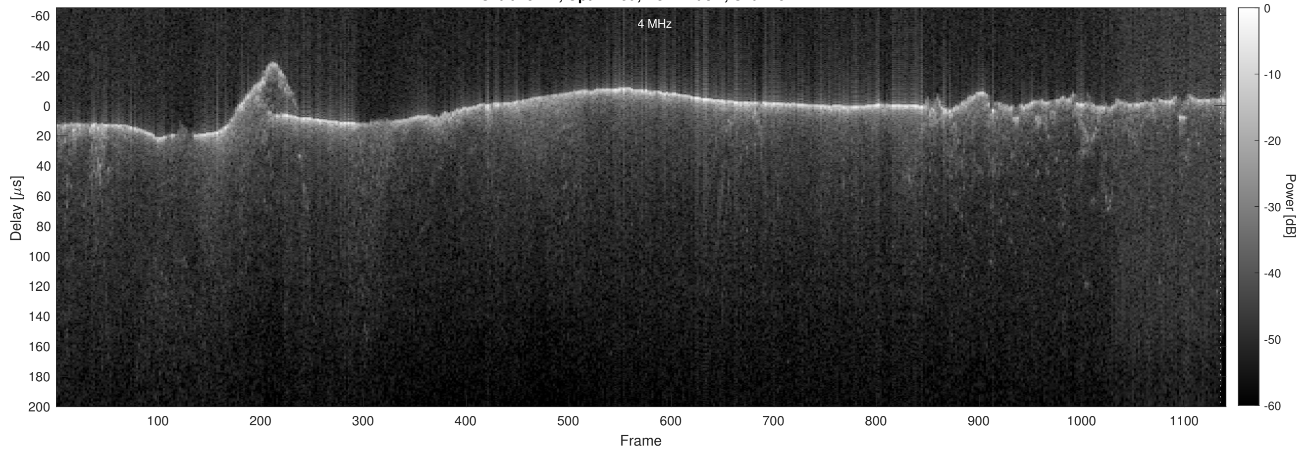
Orbit 15472, Optimized, No Window, Channel 2
