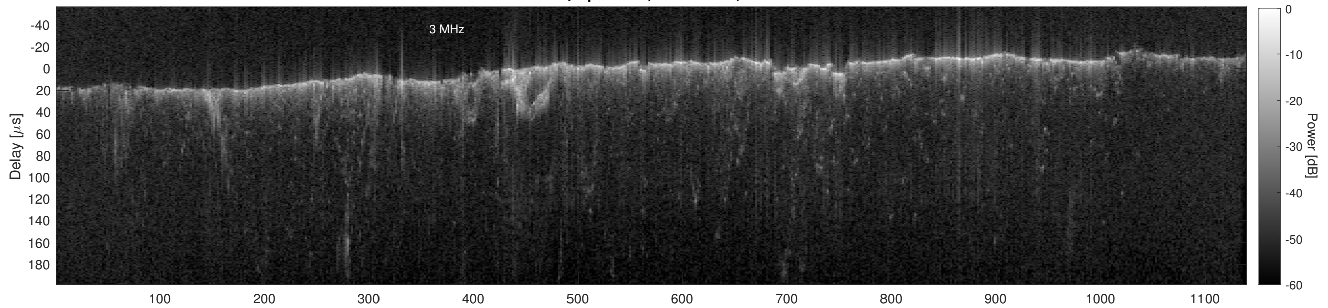
Orbit 15474, Cluttergram
