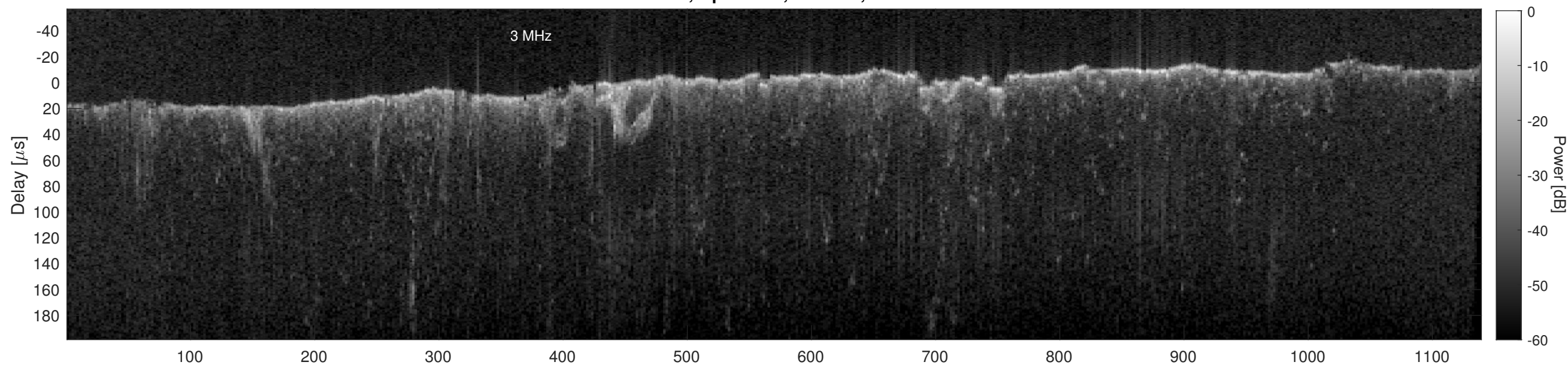
Orbit 15474, Cluttergram
