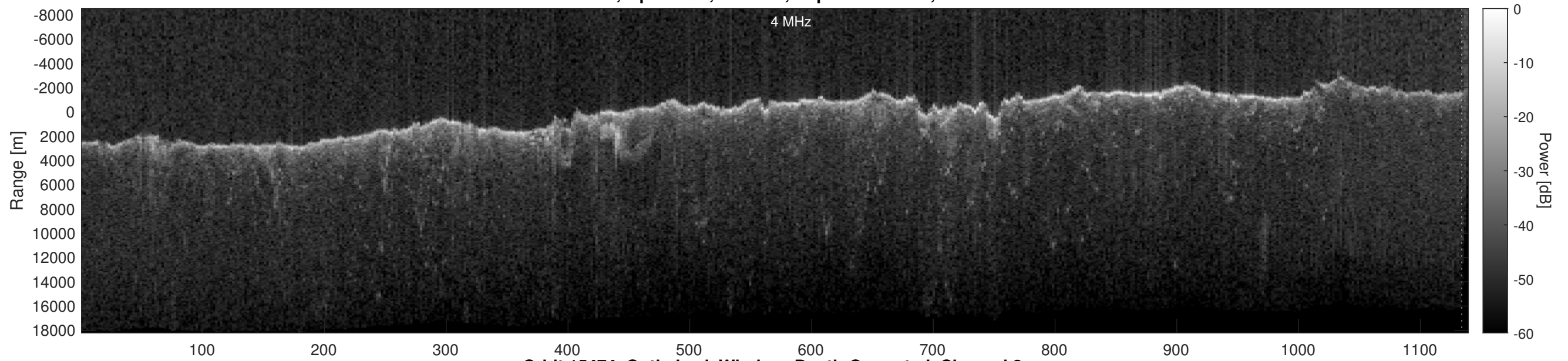
Orbit 15474, Optimized, Window, Depth-Corrected, Channel 2
