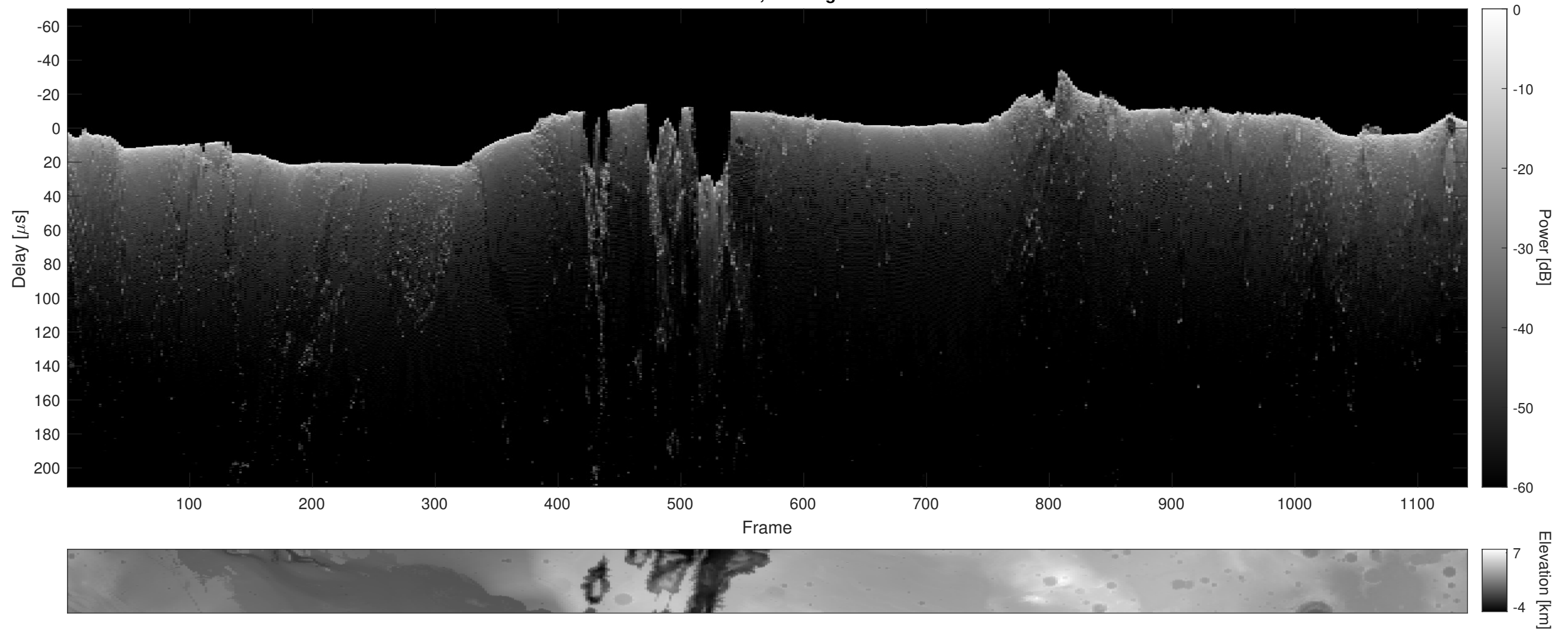
Orbit 15475, Cluttergram
