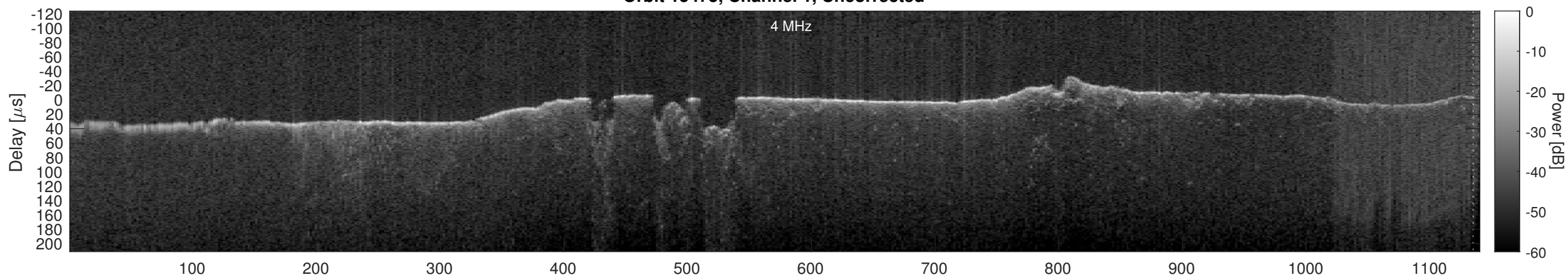
Orbit 15475, Window, Channel 1, Chapman
