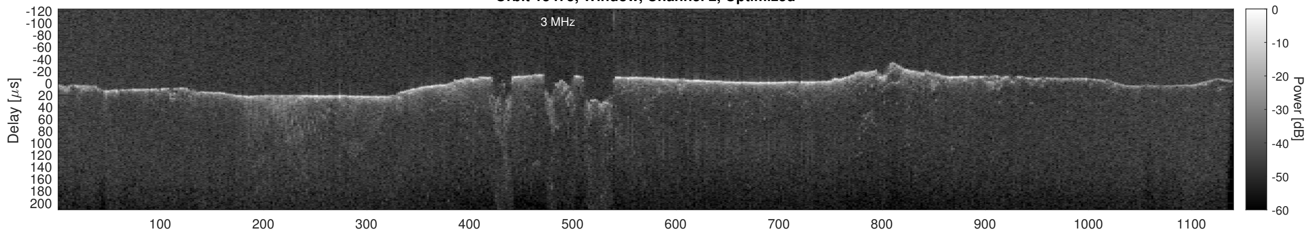
Orbit 15475, Cluttergram
