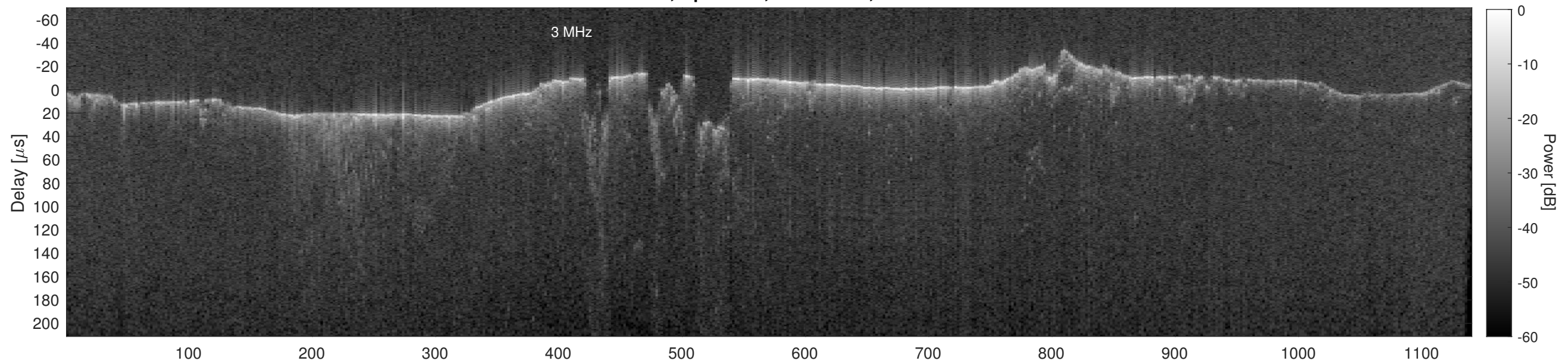
Orbit 15475, Cluttergram
