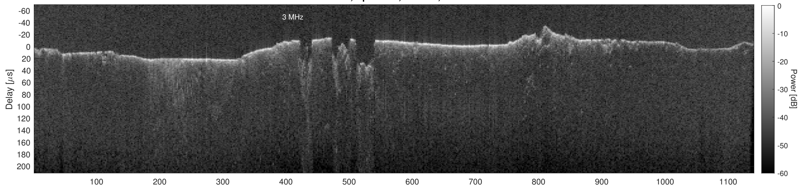
Orbit 15475, Cluttergram
