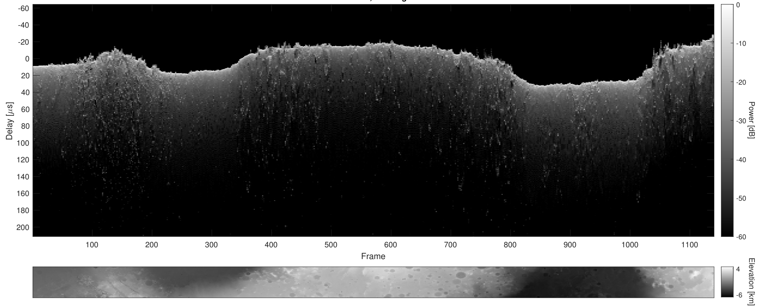
Orbit 15477, Cluttergram
