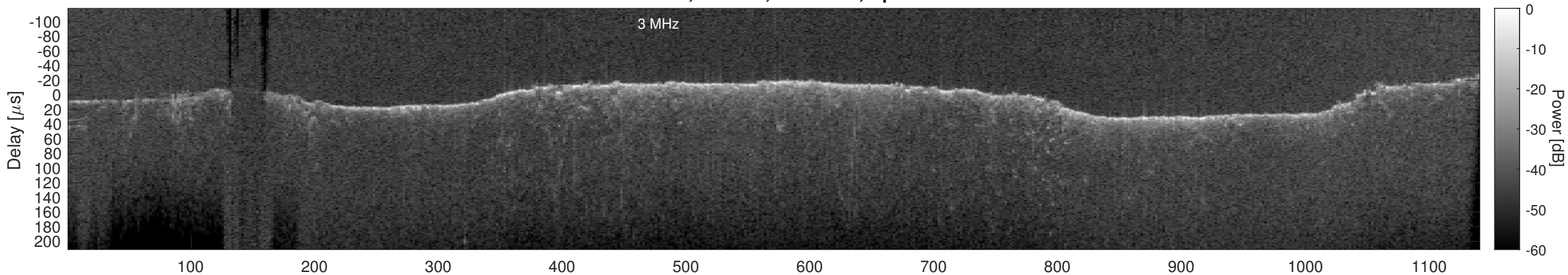
Orbit 15477, Cluttergram
