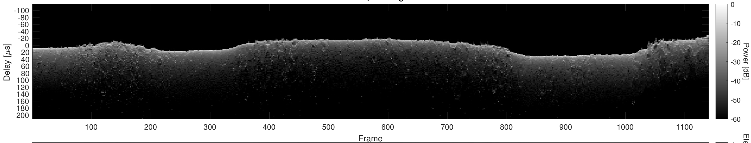
Orbit 15477, Cluttergram
