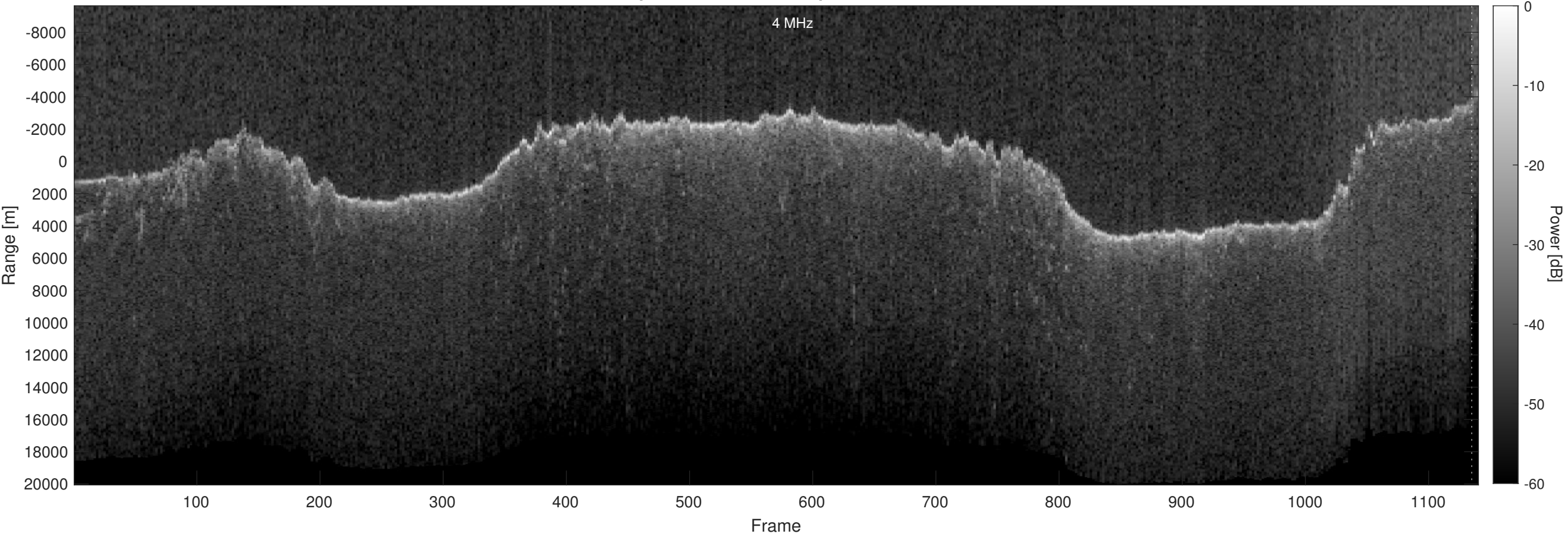
Orbit 15477, Optimized, Window, Depth-Corrected, Channel 2
