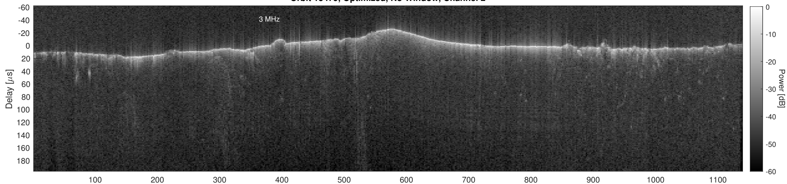
Orbit 15479, Cluttergram
