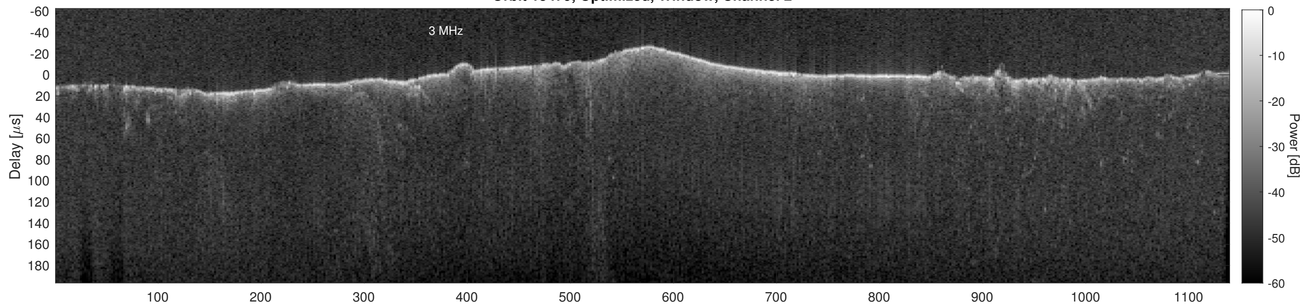
Orbit 15479, Cluttergram
