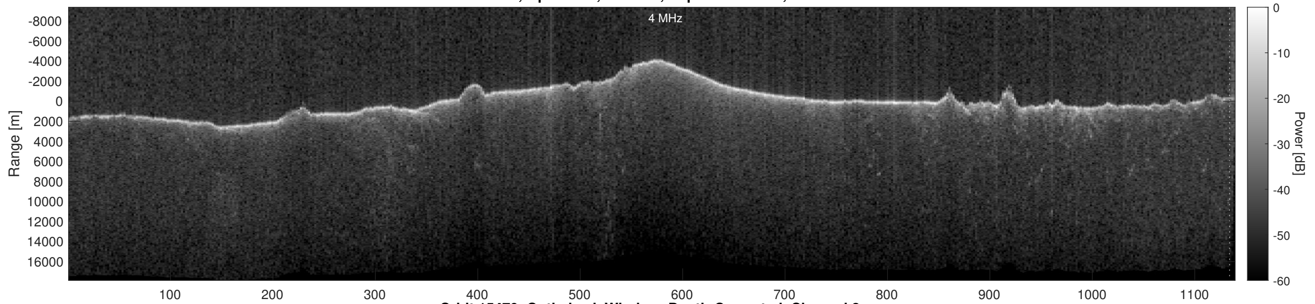
Orbit 15479, Optimized, Window, Depth-Corrected, Channel 2
