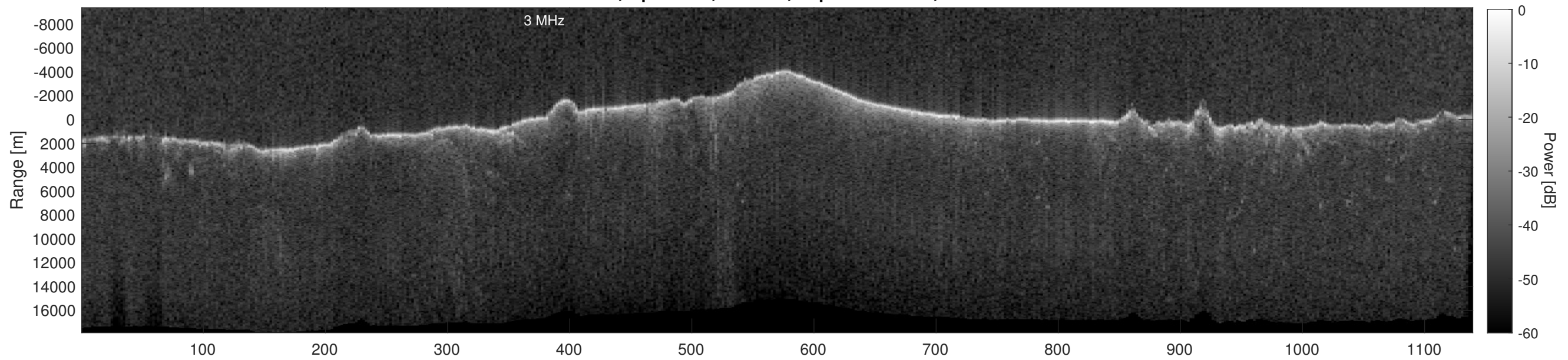
Orbit 15479, Depth-Corrected Cluttergram
