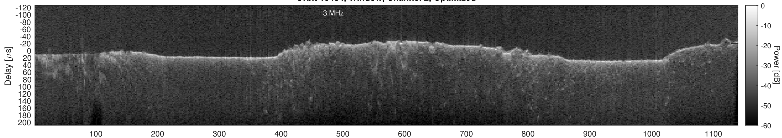
Orbit 15484, Cluttergram
