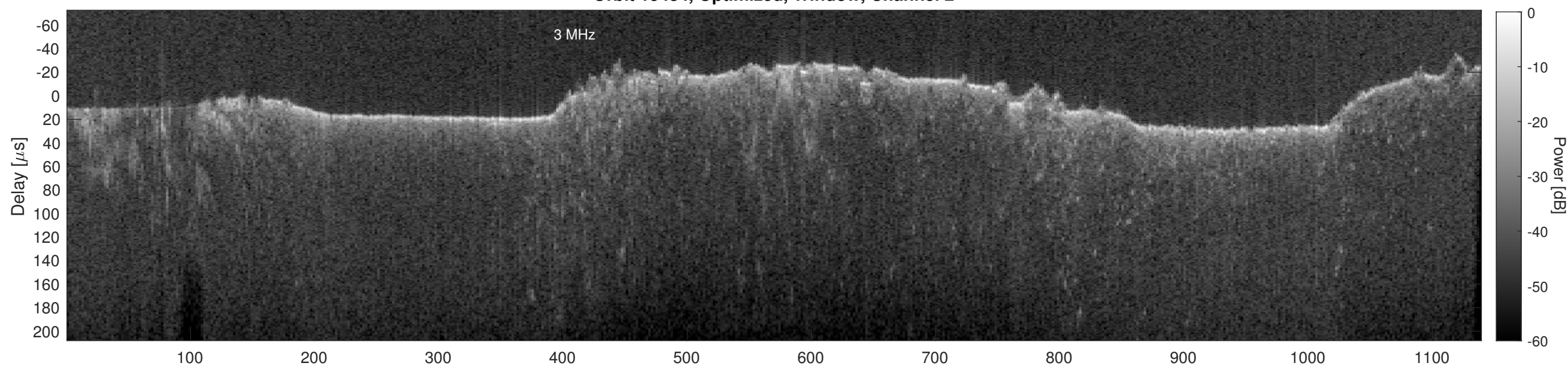
Orbit 15484, Cluttergram
