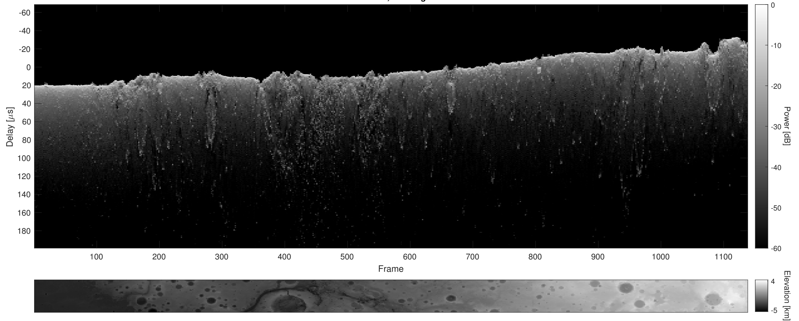
Orbit 15485, Cluttergram
