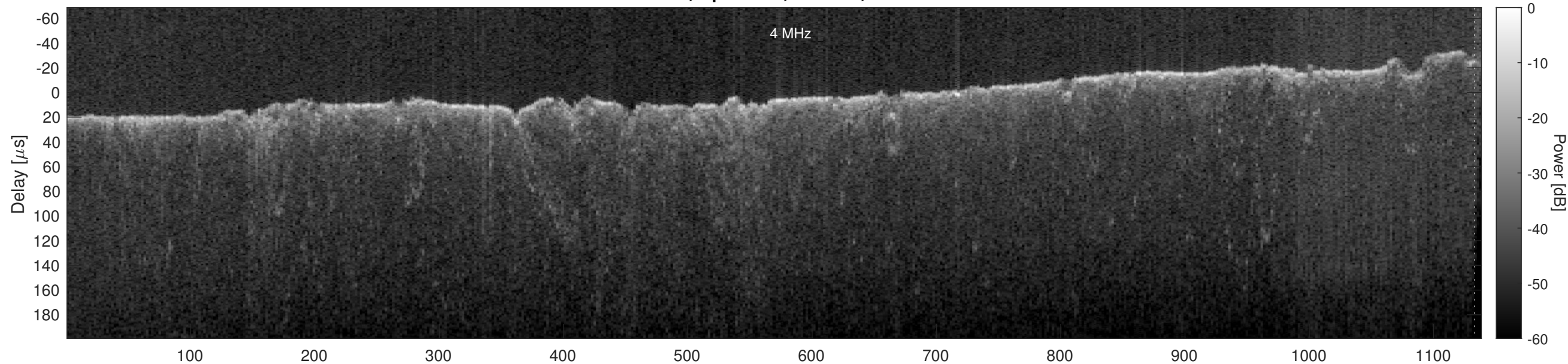
Orbit 15485, Optimized, Window, Channel 2
