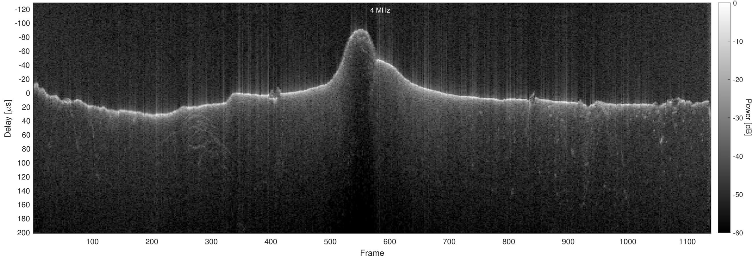
Orbit 15486, Chapman, No Window, Channel 2
