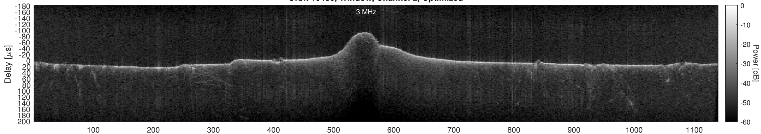
Orbit 15486, Cluttergram
