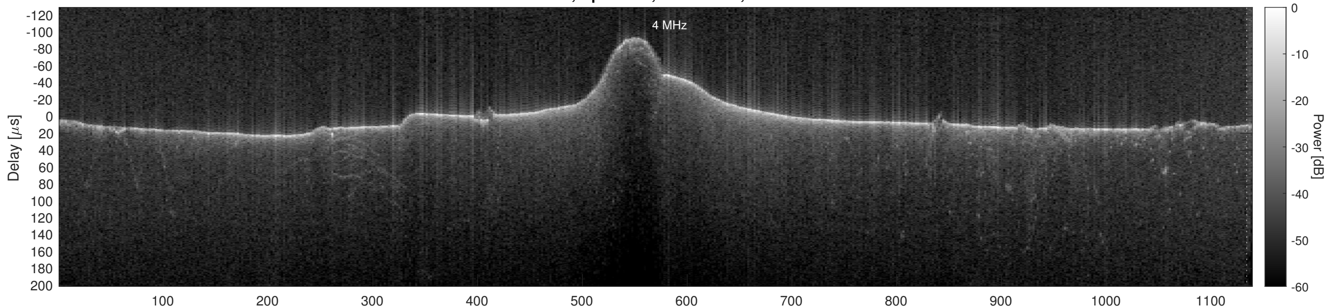
Orbit 15486, Optimized, No Window, Channel 2
