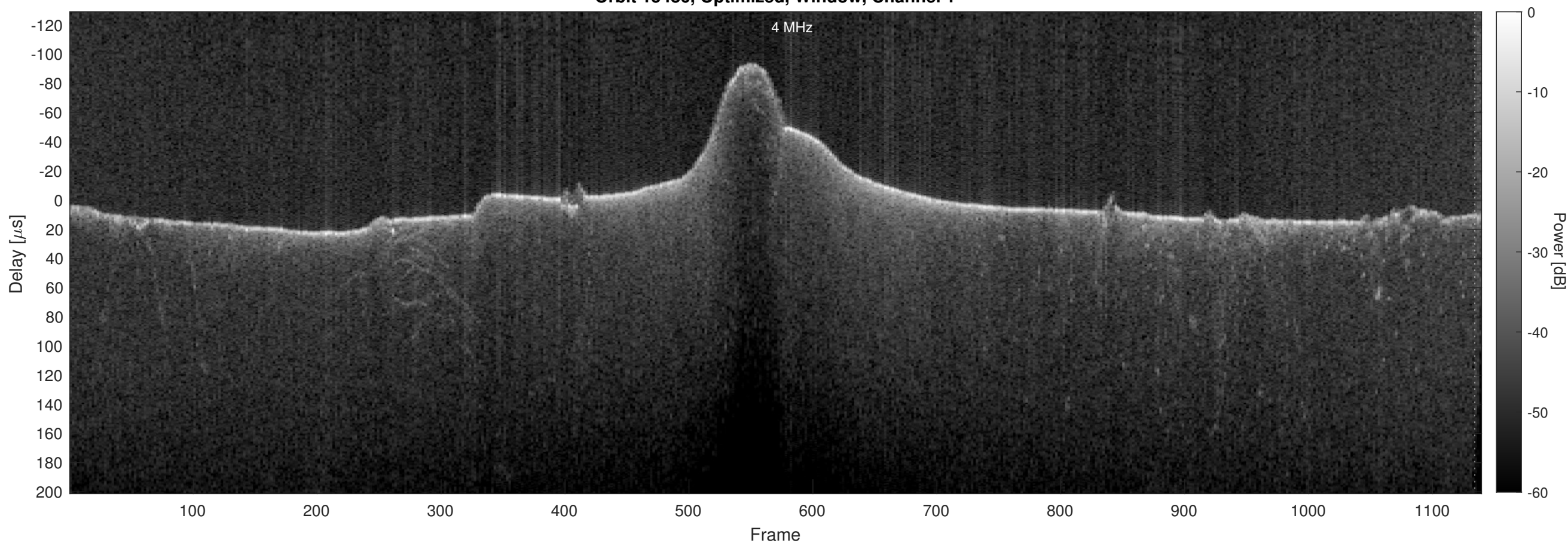
Orbit 15486, Optimized, Window, Channel 2
