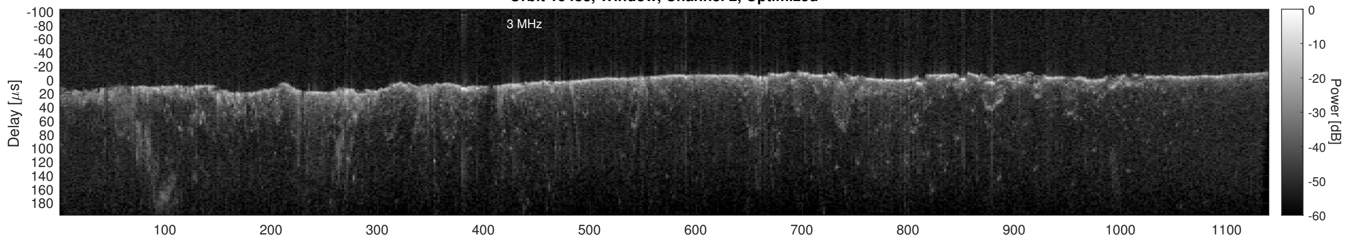
Orbit 15488, Cluttergram
