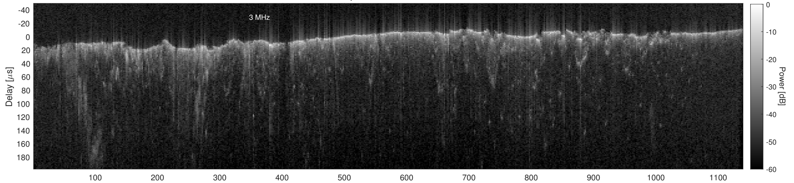
Orbit 15488, Cluttergram
