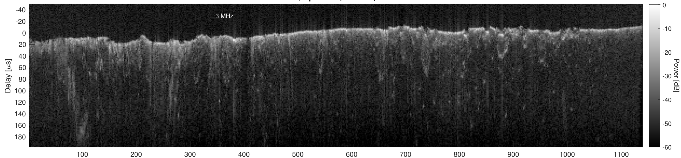
Orbit 15488, Cluttergram
